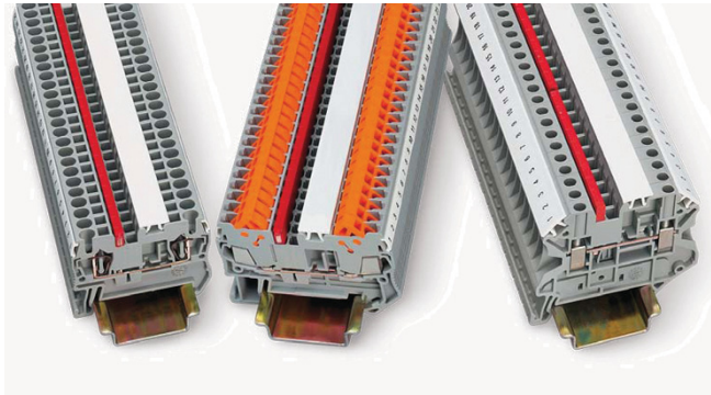
IEC—XB Series
